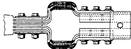
Flexible connector with special tinned length and drilling.
