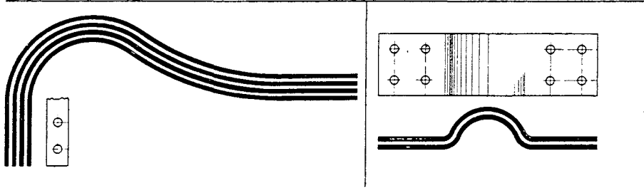
Assembly of expansion joint for three inch hollow square channel bus.
