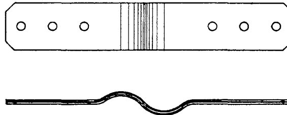
Flexible connector with special tinned length and drilling.
