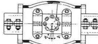
TYPE GCE (Page Fa-3)
